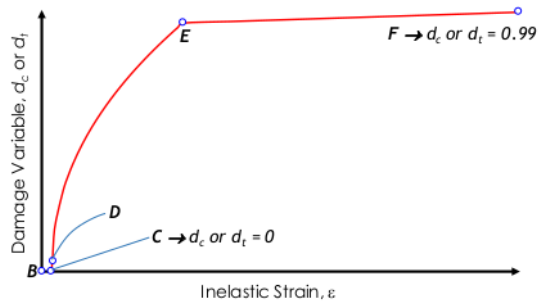
Typical damaged parameter for concrete [19]
