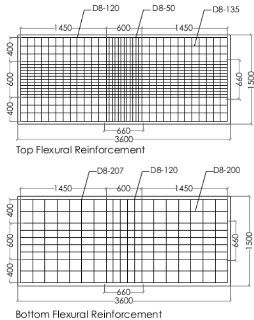
Figure 2 Slab reinforcement layouts by Gunadi et al. [14]
