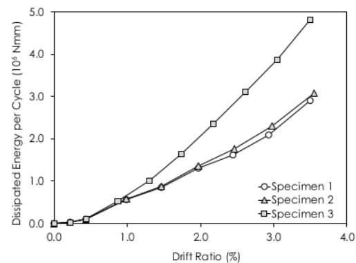
Figure 10 Energy dissipation up to drift ratio of 3.5%
