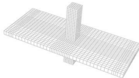
Figure 4 Mesh configuration of numerical model
