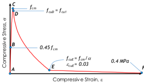
Compressive behavior for concrete [19]
