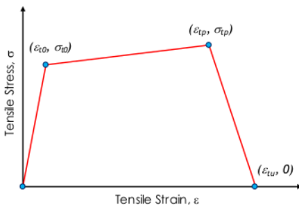
Tensile stress-strain for PVA-ECC material [23]
