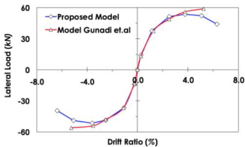
Figure 7 Verified backbone curve of experimental work
