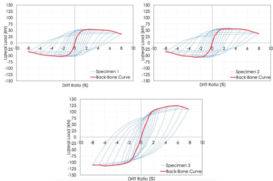
Figure 8 Hysteresis curves of all specimens
