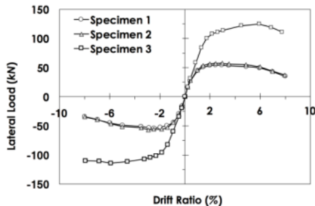
Figure 9 Backbone curves of all specimens
