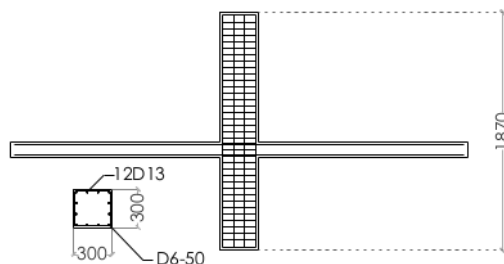
Figure 3 Column rebar layouts by Gunadi et al. [14]
