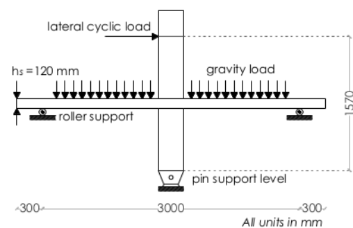
Figure 1 Geometry of specimen by Gunadi et al. [14]
