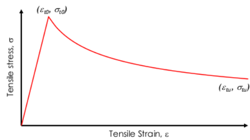
Tensile behavior for concrete [18]
