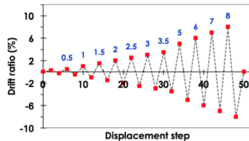
Figure 5 Pattern of lateral cyclic load
